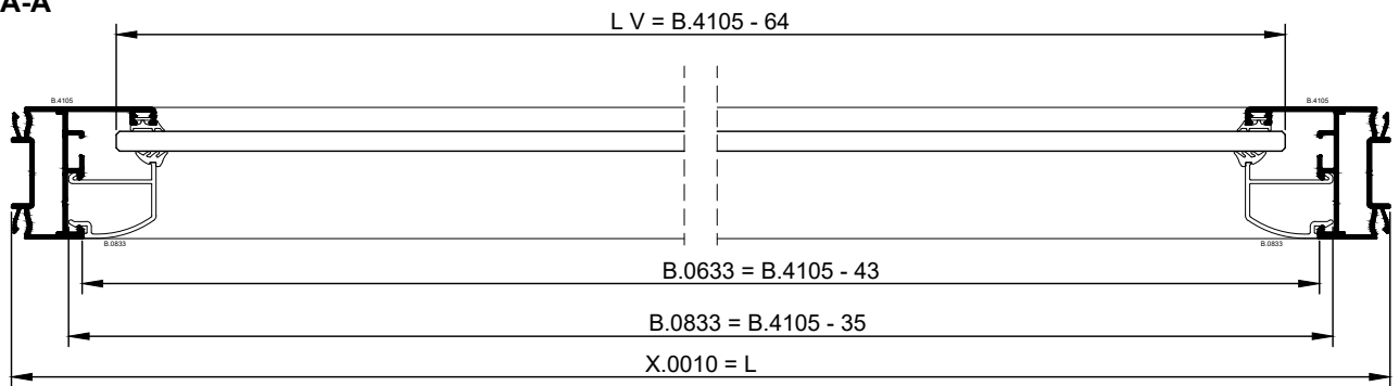
SEC. C-C
