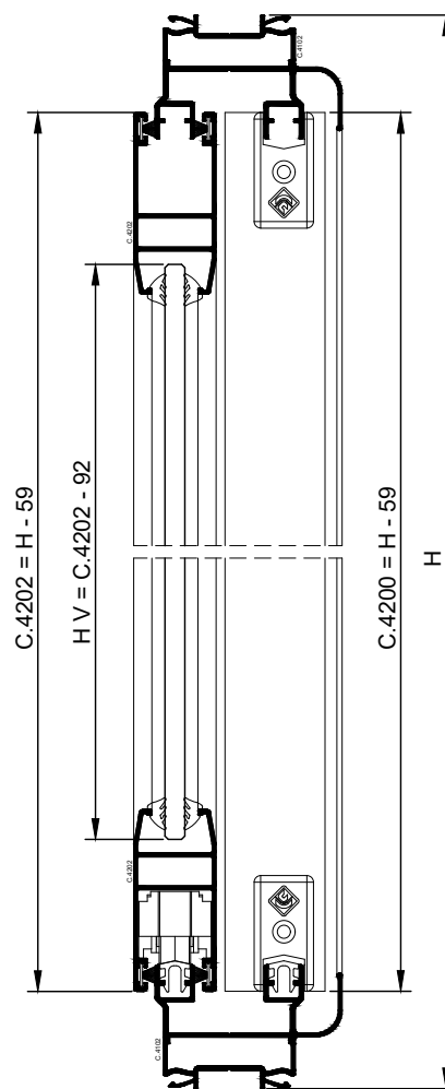
SEC. B-B
